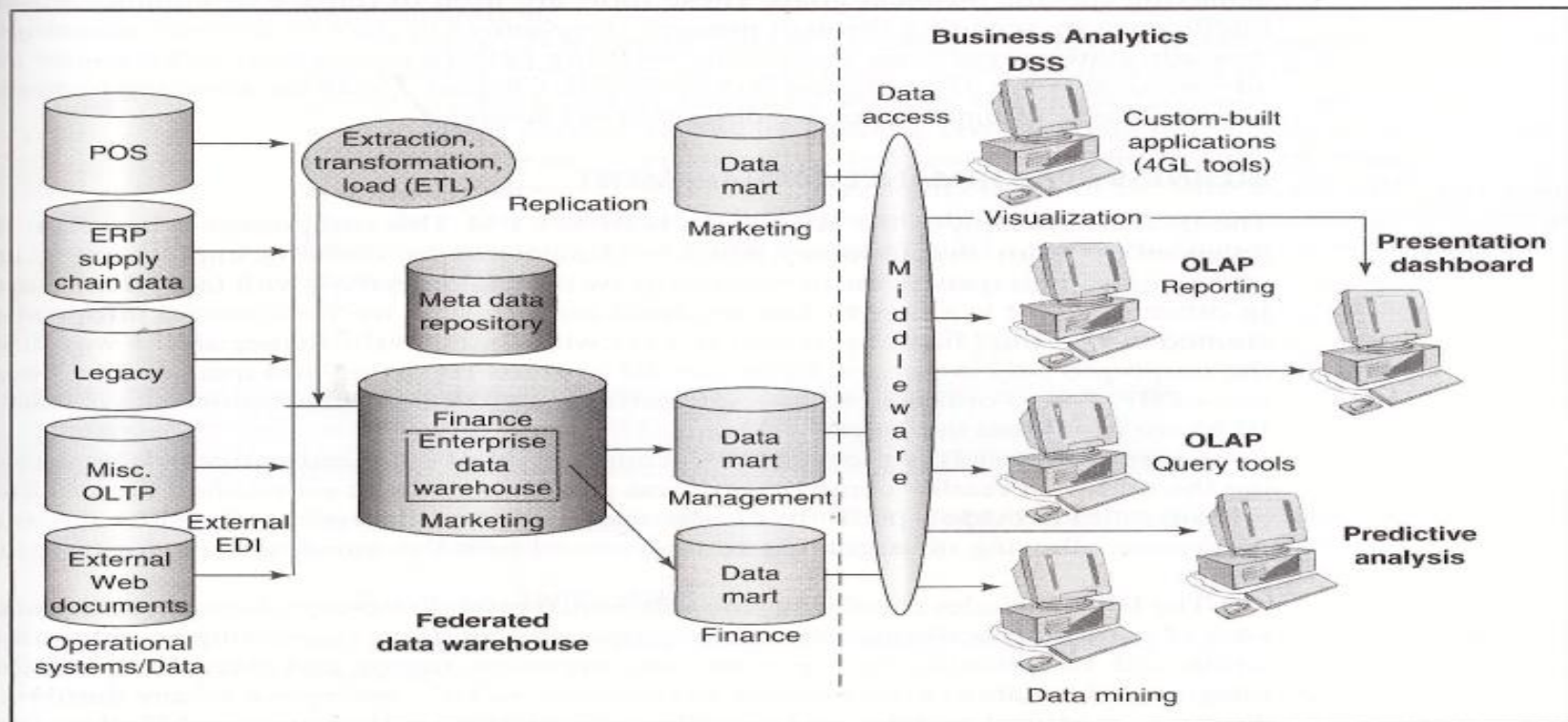
FIGURE S.4 The Major Components of Business Intelligence
